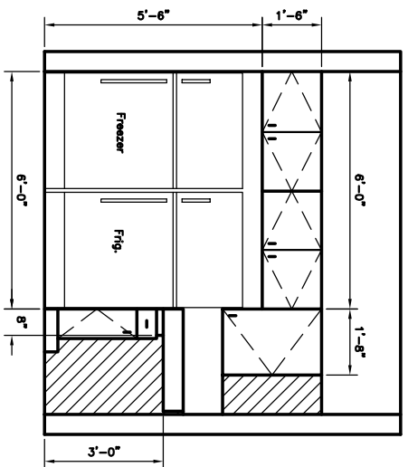
Ⓢ BUTLER'S PANTRY FREEZER SCALE: 1/2"=1'-0"
